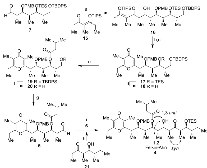
Scheme 3. Reagents and conditions: a) 15 , LDA, -78^\circ\text{C} , 7 , 94%; b) DMP, \text{CH}_2\text{Cl}_2 , \text{NaHCO}_3 ; c) DMF, 55^\circ\text{C} , 6 h, 68% over two steps; d) PPTS, \text{CH}_2\text{Cl}_2/\text{MeOH} (3:1), 96%; e) 2,4,6-trichlorobenzoyl chloride, DMAP, \text{Et}_3\text{N} , isovaleric acid, 98%; f) \text{HF}\cdot\text{py} , \text{CH}_3\text{CN}/\text{py} (7:1), 94%; g) DMP, \text{CH}_2\text{Cl}_2 , \text{NaHCO}_3 , 98%; h) \text{TESCl} , imidazole, \text{CH}_2\text{Cl}_2 , 96%; i) 6 , c\text{Hex}_2\text{BCl} , \text{Me}_2\text{NEt} , \text{Et}_2\text{O} , -78^\circ\text{C} \rightarrow 0^\circ\text{C} , 2 h; 0^\circ\text{C} \rightarrow -78^\circ\text{C} ; 5 , -78^\circ\text{C} \rightarrow -25^\circ\text{C} , 15 h; \text{H}_2\text{O}_2 , \text{MeOH} , pH 7 buffer, 0^\circ\text{C} , 1 h, 94%, 21:1 d.r. TIPS = triisopropylsilyl, LDA = lithium diisopropylamide, DMP = Dess-Martin periodinane, DMF = N,N -dimethylformamide, PPTS = pyridinium para -toluenesulfonate, DMAP = 4-dimethylaminopyridine, py = pyridine.
